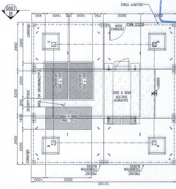
A PROPOSED SITE LAYOUT NTS SCALE: 1:1
